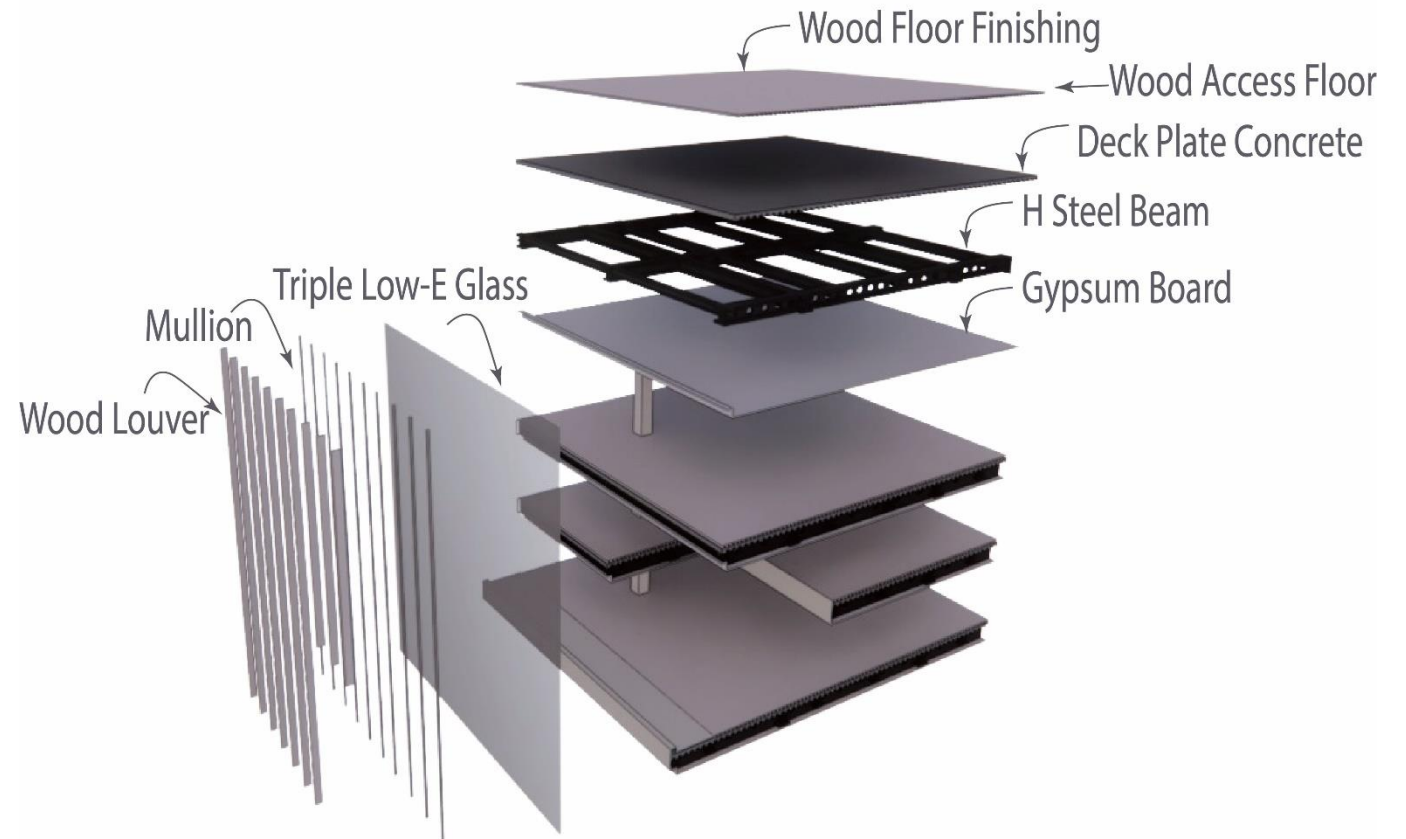
Exploded Axonometric
