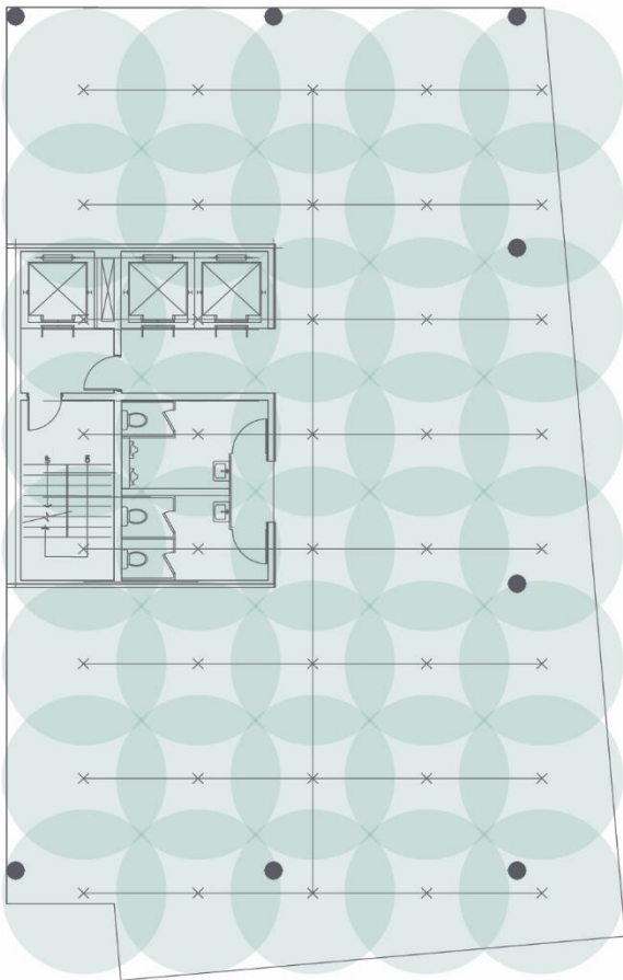
Sprinkler Plan
